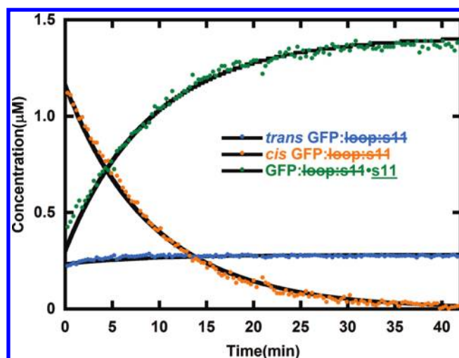
Figure 6. The evolution of concentrations of trans -GFP:Δs11 (blue), cis -GFP:Δs11 (yellow), and GFP:Δs11•s11 (green) after generating a photostationary mixture of cis - and trans -GFP:Δs11 and mixing in s11. The solid black lines are generated by the model in Figure 3 (a unimolecular reaction of cis converting back to trans -GFP:Δs11, and a bimolecular reaction of s11 forming a complex with cis -GFP:Δs11). As expected from this model, the cis GFP:Δs11 concentration drops as the other species rise, and after the cis -GFP:Δs11 is gone the concentrations of trans -GFP:Δs11 and GFP:Δs11•s11 remain constant. If the sample is excited with additional light, the reassembly can be driven to completion (data not shown). The initial concentrations of trans -GFP:Δs11 and s11 in this experiment were 2 μM and 10 μM, respectively, and they were in pH 8 buffer at 18 °C.
