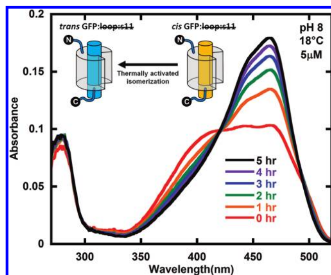
Figure 2. Reformation of trans -GFP:loop:s11 (compare final black spectrum with Figure 1B) in the dark after creating the photostationary state of trans - and cis -GFP:loop:s11 (red) with 460 nm light. The sample was kept rigorously in the dark and the absorbance spectrum sampled infrequently. The cartoons show the part of the kinetic model that describes this data. The protein was at a concentration of 5 \mu M in pH 8 buffer at 18 ^{\circ} C. See Figure 5 for kinetics as a function of temperature.
