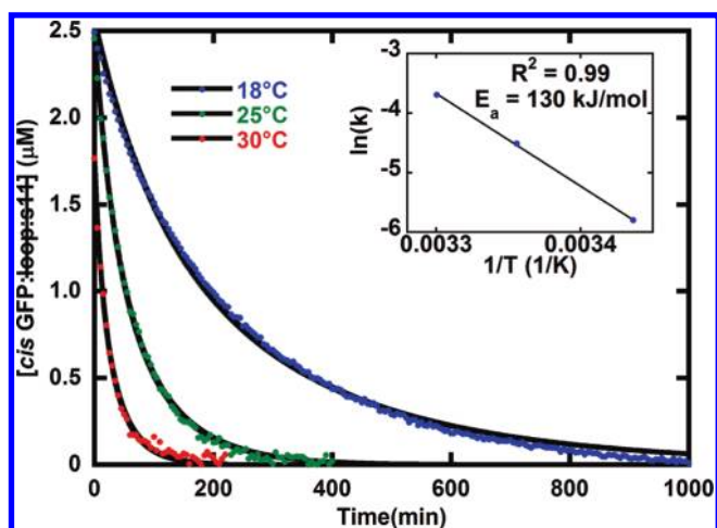
Figure 5. Temperature dependence of the decay of cis -GFP:Δs11 from the photostationary state to form the more stable trans -GFP:Δs11. The red, green, and blue dots show the concentration decrease in time after the light-activated generation of cis -GFP:Δs11 at 30 °C, 25 °C, and 18 °C, respectively. The solid black line fits are obtained from fitting the concentrations of all species with the kinetic model shown in Figure 2 (a unimolecular reaction of cis -GFP:Δs11 converting back to trans -GFP:Δs11 and a bimolecular aggregation of cis -GFP:Δs11; see Supporting Information). Inset: The temperature dependence shows Arrhenius behavior with an activation energy of 130 kJ/mol. All three samples had a total protein concentration of 5 μM and were in pH 8 buffer.
